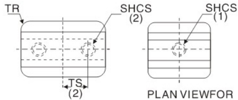
PLAN VIEW FOR UULG 2001 & 4001 AND TTAM 100 & TTGU25
